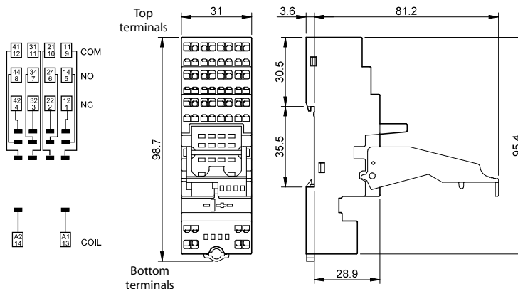
Sockets + jumper link
