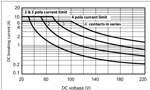
H 55 - Maximum DC1 breaking capacity
